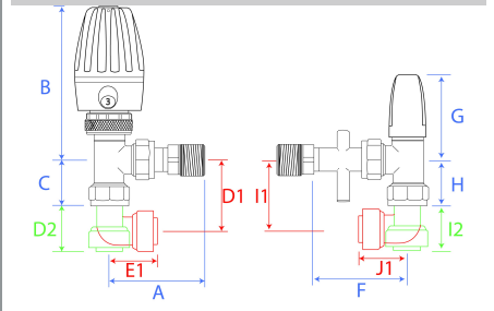
TRV & Drain Off Lockshield Pack
